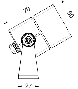
Physical Dimension(MM)
