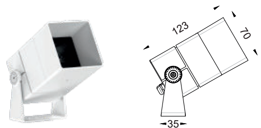
Cuboid hood
