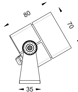
Physical Dimension(MM)
