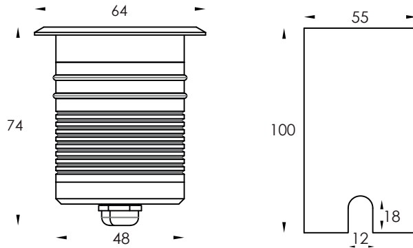
Physical Dimension(MM)
