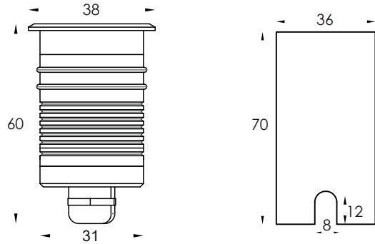
Physical Dimension(MM)
