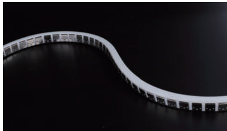
Stainless Flexible Profile Item No : JK0022 Dimension(LxWxH) : 970 X 20.2 X 10.8mm Material : SUS304\SUS316
